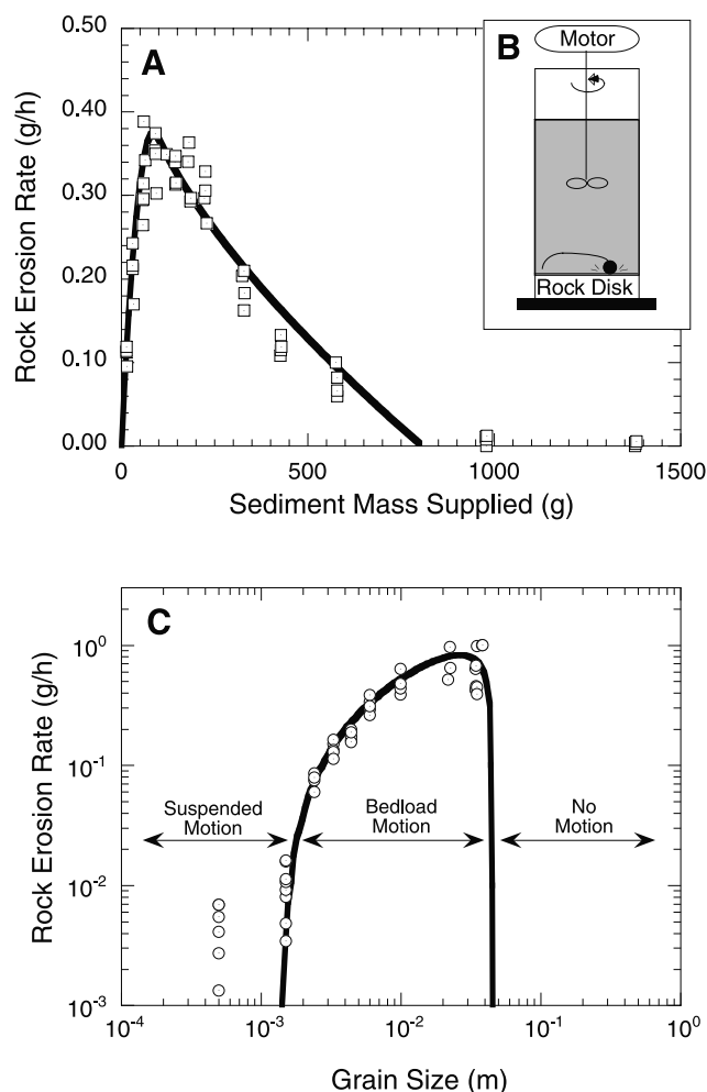
Figure 10. Experimental results demonstrating sediment supply and grain size effects on rates of bedrock wear, shown in grams per hour (g/h). A. Variation in wear rate with sediment supply using the apparatus shown in B. Erosion rate increases with sediment additions until bed armoring by immobile sediment reduces the area of exposed bedrock. Erosion rate declines with further sediment additions until bed is fully buried. C. Wear rate variation with grain size. Wear rate declines with decreasing grain size because of a tendency for small grains to go into suspension and reaches a peak at a grain size that is just above the threshold of motion.
