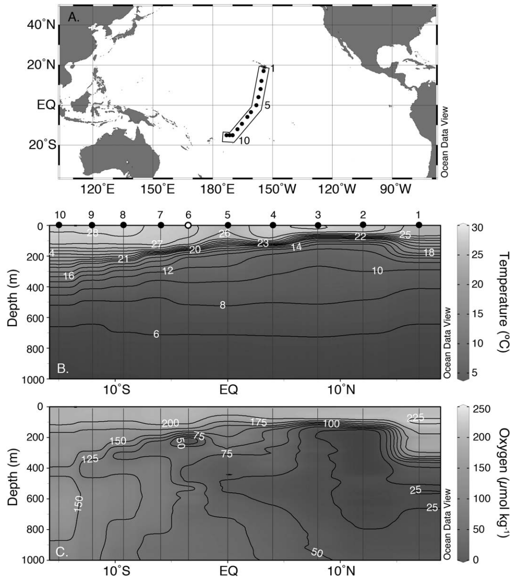
Fig. 1. (A) Location of the METZYME cruise across the equatorial Pacific. (B) Temperature and (C) oxygen concentration across the cruise track. Temperature and oxygen data are reported as 1 m-binned averages from the CTD sensors. Station locations are indicated as black circles with station numbers above. Open circle denotes a station where only physicochemical samples (i.e., no molecular samples) were collected (station 6). Data were contoured using weighted-average gridding in Ocean Data View v4.7.3.
