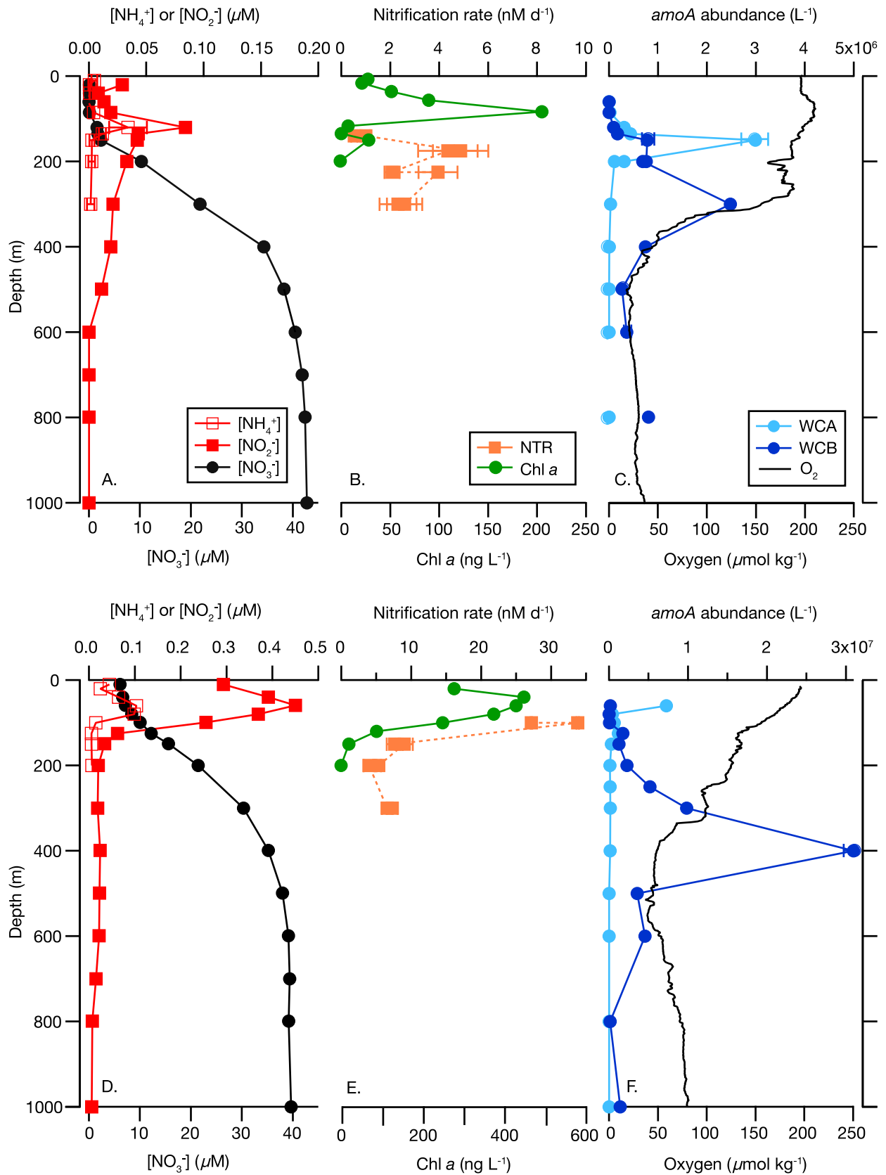
Fig. 2. Representative depth profiles from station 1 (17° N, top row) and station 5 (Equator, bottom row) ( A, D ). [\text{NH}_4^+] (open squares), [\text{NO}_2^-] (filled squares), [\text{NO}_3^-] (filled circles). Error bars for [\text{NH}_4^+] measurements represent standard error of triplicate measurements and in most cases are smaller than the symbol ( B, E ). Nitrification rates (NTR) determined using ^{15}\text{NH}_4\text{Cl} (filled squares) and Chl a determined using high performance liquid chromatography (filled circles). Error bars for NTR indicate standard error in the model fit, and in most cases are smaller than the symbol; ( C, F ). Abundance of archaeal amoA genes determined using qPCR for the water column "A" (WCA) and water column "B" (WCB) ecotypes, and dissolved oxygen. Points are the mean of triplicate qPCR analyses; error bars indicate standard deviation from the mean and in most cases are smaller than the symbol. Note that scaling changes on most horizontal axes between stations.
