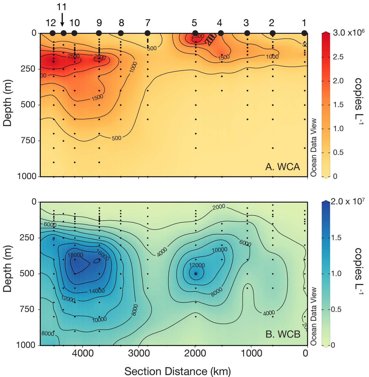
Fig. 4. Abundance of archaeal amoA genes in the equatorial Pacific between W. Samoa (section distance ~ 5000 km) and offshore of Hawai'i (section distance ~ 0 km) as determined by quantitative PCR (qPCR). (A) Water column "A" (WCA) clade, (B) water column "B" (WCB) clade. Station numbers are indicated along the top of panel A . Note the x-axis differs slightly from Fig. 1 to display data from multiple stations occupied along 15°S (see Fig. 1A), and that the color scale range is different for panels A and B . Points below the detection limit of our qPCR assays were coded as zero values for data interpolation using the weighted-average gridding algorithm in Ocean Data View v4.7.3 with automatic x and y scale lengths.
