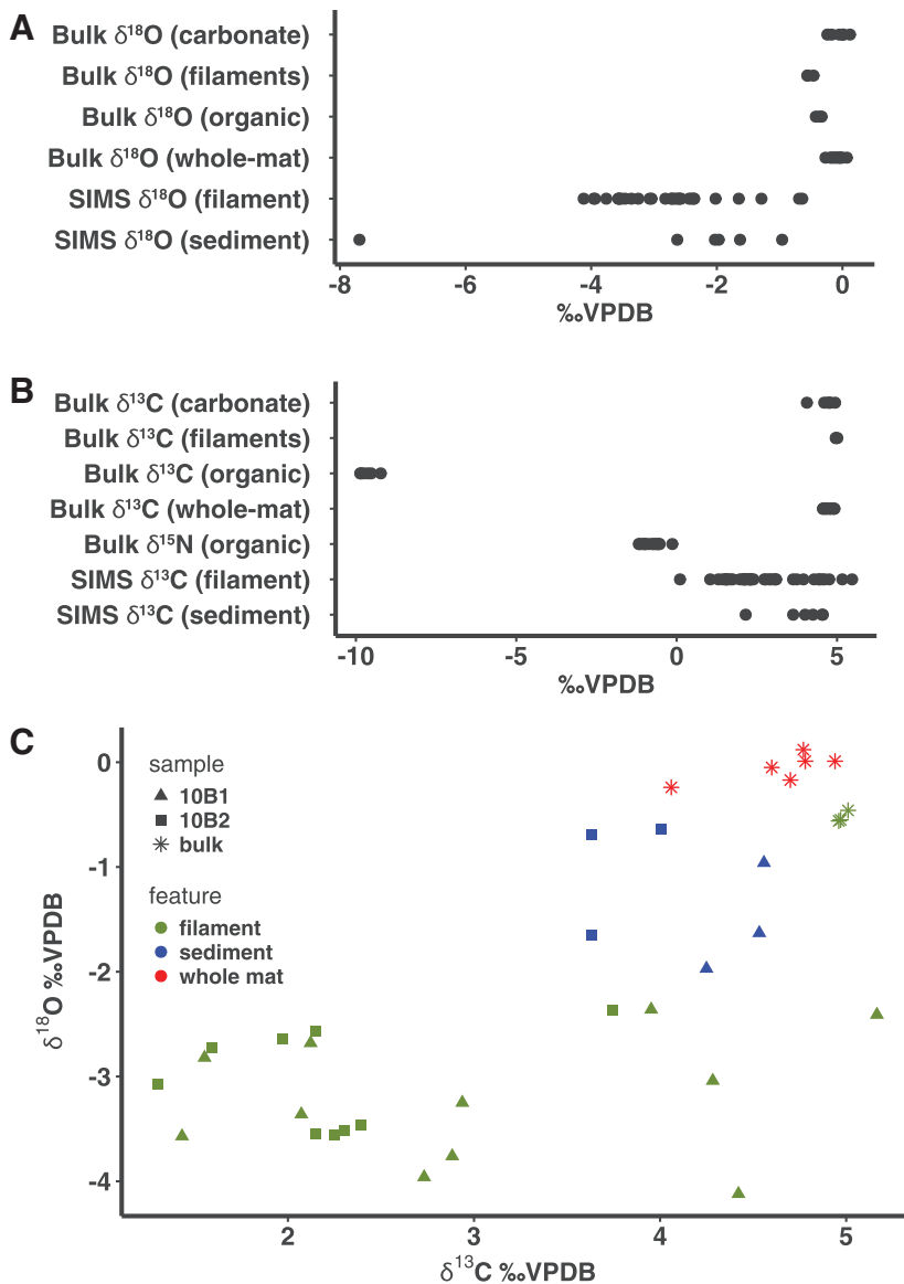
FIG. 7. Stable isotope results for calcified filaments located in the upper 3 mm of thrombolite-forming button mat. (A) Oxygen isotope values of organic and inorganic fractions using both bulk and SIMS analysis. Analyses were completed for both background carbonate precipitates (sediment), calcified filaments (filaments), and untreated whole mat samples. (B) Carbon and nitrogen isotope values of both organic and inorganic fractions using both bulk and SIMS analysis. (C) Comparative plot of SIMS values collected for oxygen and carbon isotopes. All results are expressed in delta notation with respect to the carbon/oxygen Vienna Pee Dee Belemnite (VPDB) or nitrogen air (AIR) standard.
