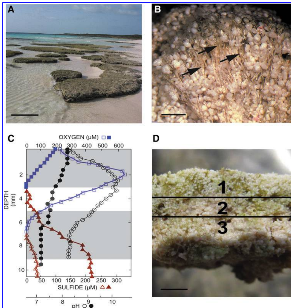
FIG. 1. The thrombolites of Highborne Cay, The Bahamas. (A) Intertidal thrombolite platforms from Site 5. Bar, 1 m. (B) Light micrograph of a thrombolite-forming button mat revealing extensive vertical assemblages of calcified filaments (arrows). Bar, 500 \mu\text{m} . (C) In situ depth profiles of oxygen (square), sulfide (triangle), and pH (circle) collected at peak of photosynthesis (open symbols) or respiration (filled symbols). Shaded areas reflect the targeted areas collected for analysis. Depths below 9 cm were not sampled, as that region shared the same biochemical profile as in Zone 3. (D) Cross section of button mat depicting the three spatial regions including an oxic Zone 1 (0–3 mm), transitional Zone 2 (3–5 mm), and anoxic Zone 3 (5–9 mm). Bar, 3 mm.
