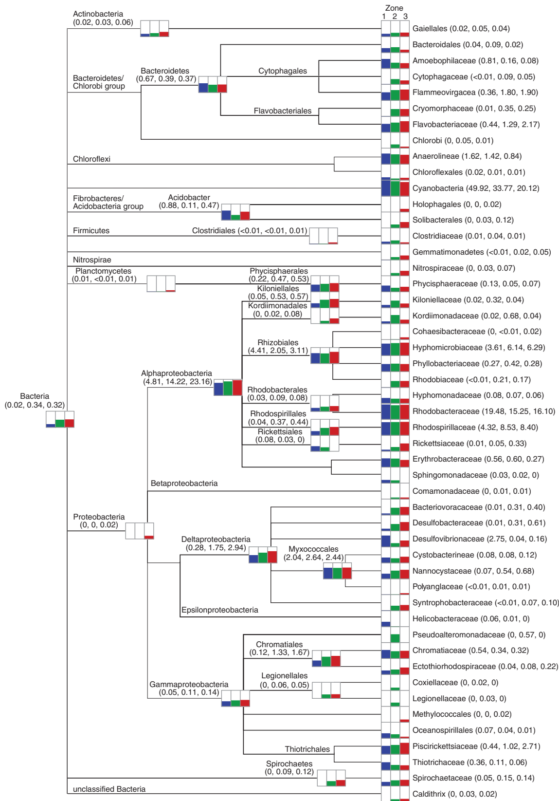
FIG. 3. Taxonomic distribution of Bacteria within the thrombolite-forming mats derived from MEGAN5 using the Greengenes database. Overall percentages based on read counts are presented logarithmically, depicting the distributions for Zone 1 (blue), Zone 2 (green), and Zone 3 (red). Read abundance data for each taxonomic level are included in parentheses.
