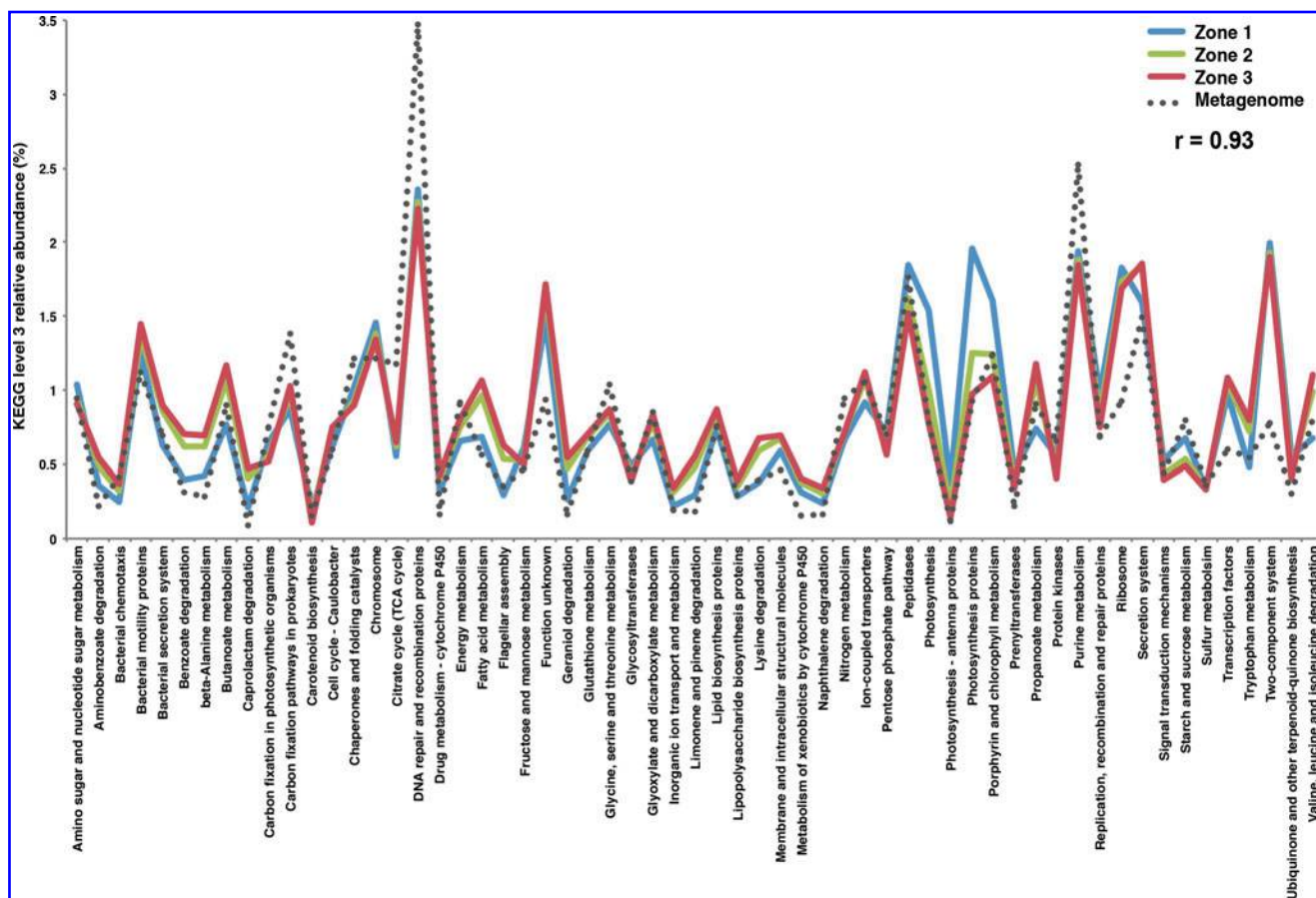
FIG. 6. Functional gene comparison of the three thrombolitic mat spatial zones from 16S rRNA metabolic prediction (PICRUST) and whole shotgun sequencing. Pearson correlation value ( r ) is shown for the comparison of metabolic predictions for Zone 1 (blue), Zone 2 (green), and Zone 3 (red) and the whole mat shotgun metagenome.
