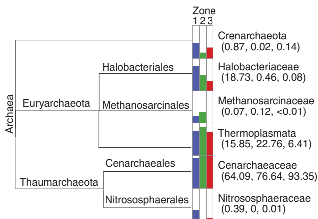
FIG. 5. Taxonomic distribution of Archaea within the thrombolite-forming mats derived from MEGAN5 using the Greengenes database. Overall percentages based on read counts are presented logarithmically, depicting the distributions for Zone 1 (blue), Zone 2 (green), and Zone 3 (red). Read abundance data for each taxonomic level are included in parentheses.
