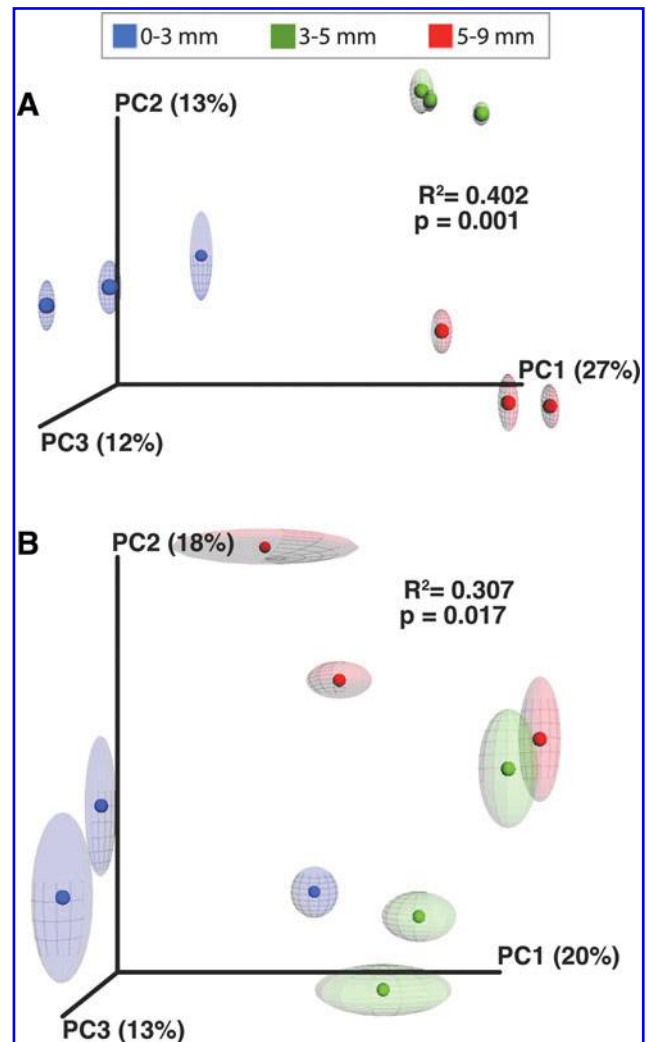
FIG. 4. Comparison of diversity analyses of three spatial zones within the thrombolite-forming mats. Principal coordinate analysis of communities from unweighted UniFrac distance matrix of Zone 1 (0–3 mm, blue), Zone 2 (3–5 mm, green), and Zone 3 (5–9 mm, red) in (A) Bacteria and (B) Archaea populations. Ellipses represent standard deviation over 10 rarefaction samplings. Adonis tests suggest that depth is a significant predictor of community composition for both bacterial ( R^2=0.402 , p=0.001 ) and archaeal ( R^2=0.307 , p=0.017 ) communities.
