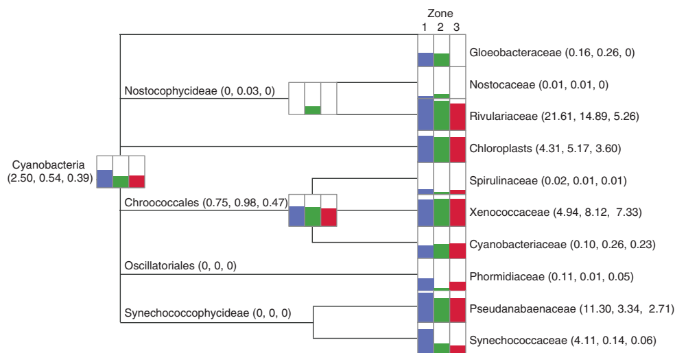
FIG. 2. Taxonomic distribution of cyanobacteria within the thrombolite-forming mats derived from MEGAN5 using the Greengenes database. Overall percentages based on read counts are presented logarithmically, depicting the distributions for Zone 1 (blue), Zone 2 (green), and Zone 3 (red). Read abundance data for each taxonomic level are included in parentheses.
