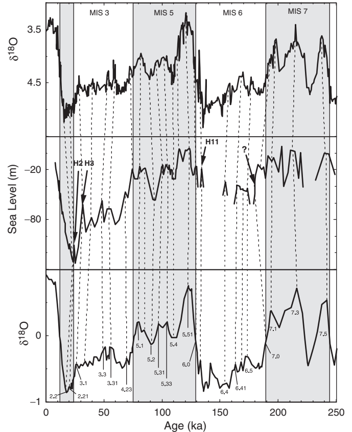
Fig. 2. Correlation of sea level and \delta^{18}\text{O} events. Dotted lines indicate correlation between records. Marine Isotope Stage boundaries indicated are those of SPECMAP. (a) The benthic \delta^{18}\text{O} record from core V19-30 (Shackleton et al., 1983), the best-resolved record in the SPECMAP stack. All \delta^{18}\text{O} scales are reversed so that negative isotopic events are peaks for ease of comparison with the sea-level record. (b) Our high-resolution coral sea-level reconstruction. Three sea-level highstands potentially associated with Heinrich events and discussed in the text are labelled. The question mark and arrow indicate an anomalous event discussed in the text. (c) The stacked SPECMAP benthic \delta^{18}\text{O} record (Pisias et al., 1984) on the SPECMAP timescale (Martinson et al., 1987) with selected \delta^{18}\text{O} events (Martinson et al., 1987) labelled.
